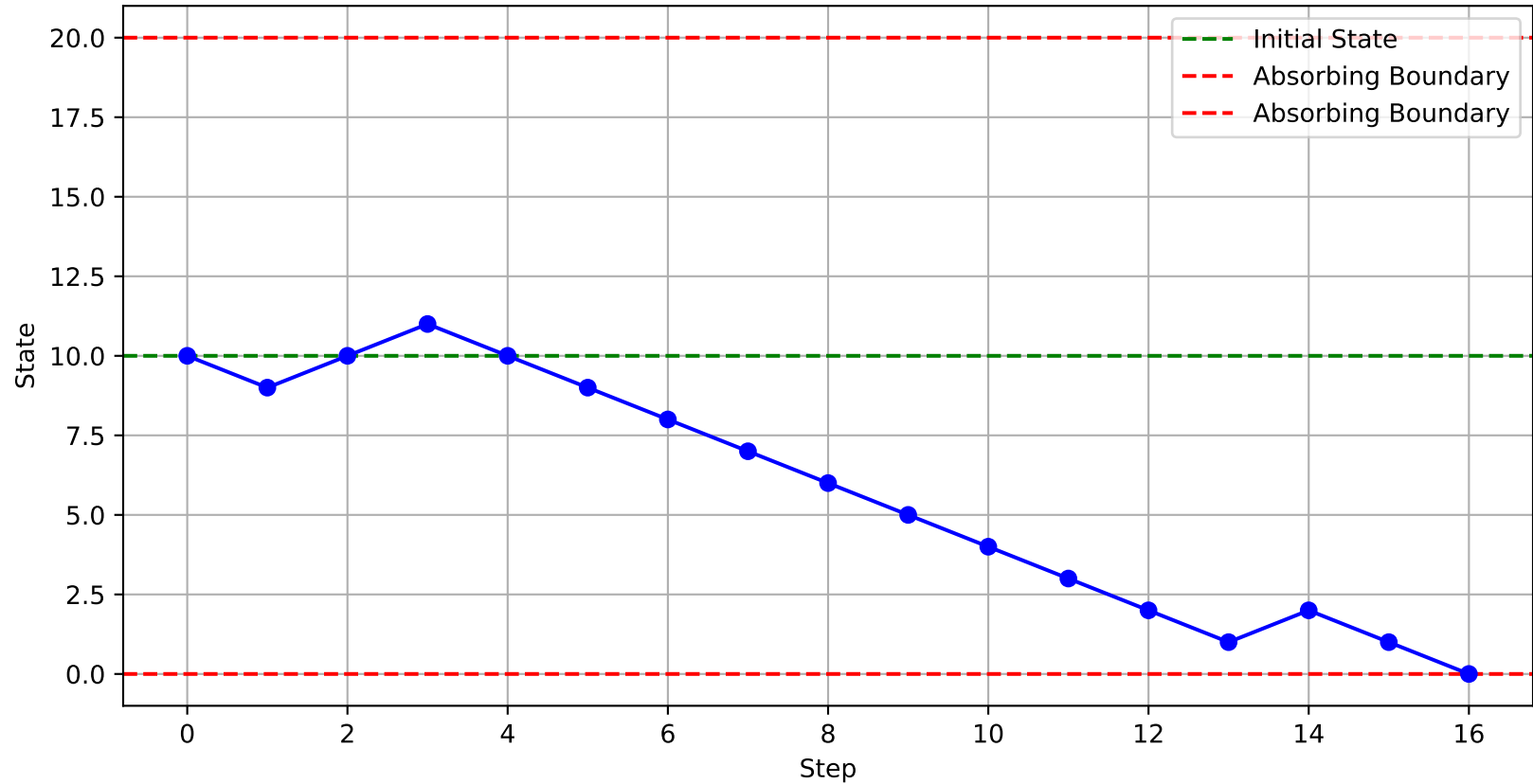
Random Walk with Absorbing Boundaries ( T=20 , p=0.5 )
